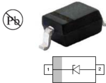
SOD-323
